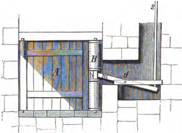
Fig. 236.—Sluice-gate.
